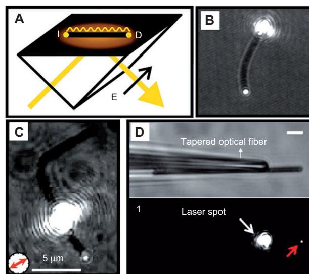
Figure 1 Optical excitation methods for surface plasmon polaritons propagating in metal nanowires [30–33].
