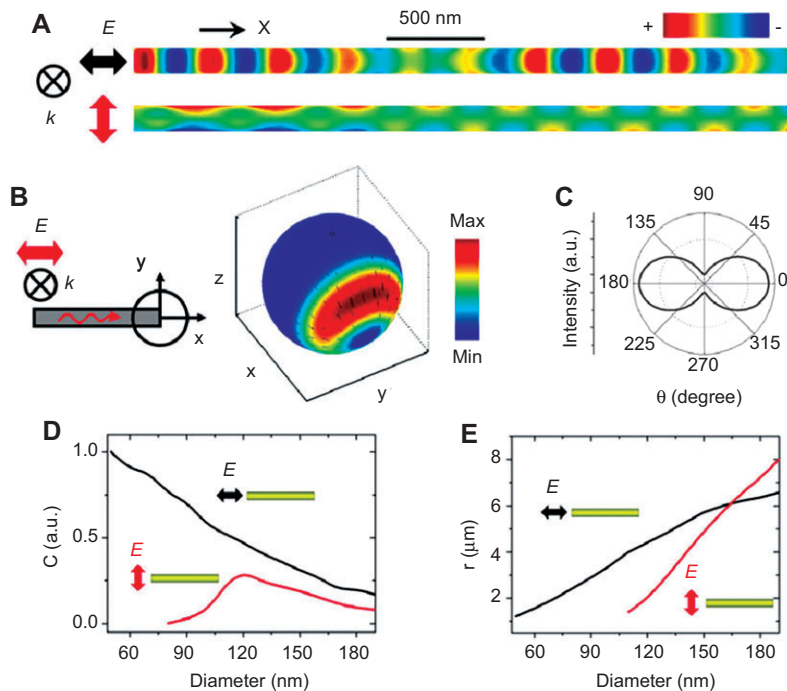
Figure 4 SPP modes in nanowires with flat terminations. (A) Charge distribution on the surface of a wire of the length 3.36 μm and diameter 130 nm, terminated by flat ends. The left end is excited by a 633 nm wavelength focused beam with polarization parallel and perpendicular to the wire, respectively. (B) The resulting spatial distribution of the emission intensity on a sphere enclosing the wire end excited by the parallel incident polarization. Colored and black lines represent the intensity and the polarization of the emission on the sphere. (C) Emission intensity of different polarizations from a wire excited under the parallel polarized excitation. (D) The in-coupling efficiency C for two SPP modes (black curve for m=0 mode, red curve for m=1 mode) as a function of the wire diameter. (E) The 1/e damping length, r , of both modes as a function of the wire diameter [43].
