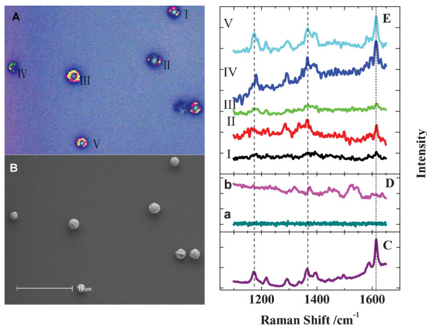
Figure 2. Optical microscopy (A) and SEM (B) images of the same flower-like silver particles. The scale bar in (B) is 10\text{ }\mu\text{m} . C) The normal Raman spectrum of the pure MGITC powder. D) The Raman spectra from individual bare silver particles without MGITC molecules. E) SERS spectra from different single flower-like silver particles marked as I–V in (A). All spectra were measured with the same accumulation time (60 s), and with 200 counts per division in (D) and (E) and 10 000 counts per division in (C).
