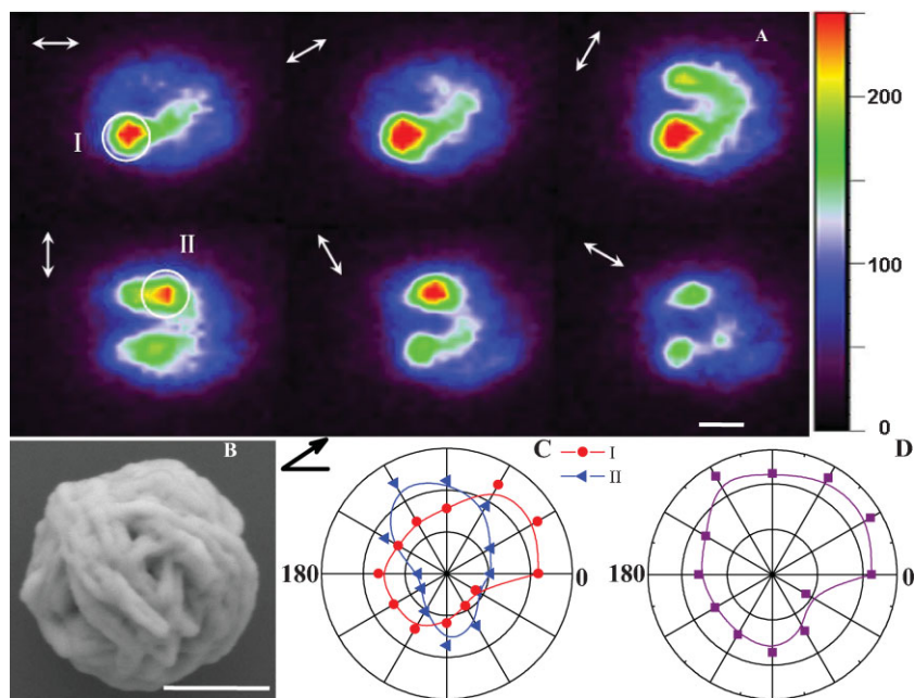
Figure 3. A) The Raman images of a single Ag nanoflower for different incident polarizations. The arrows show the different polarizations. B) The corresponding SEM image of a single particle. C) Polar plots of the Raman intensities of spot I and II marked in (A). D) Polar plots of total Raman intensity from the whole particle. All scale bars are 1 \mu\text{m} .
