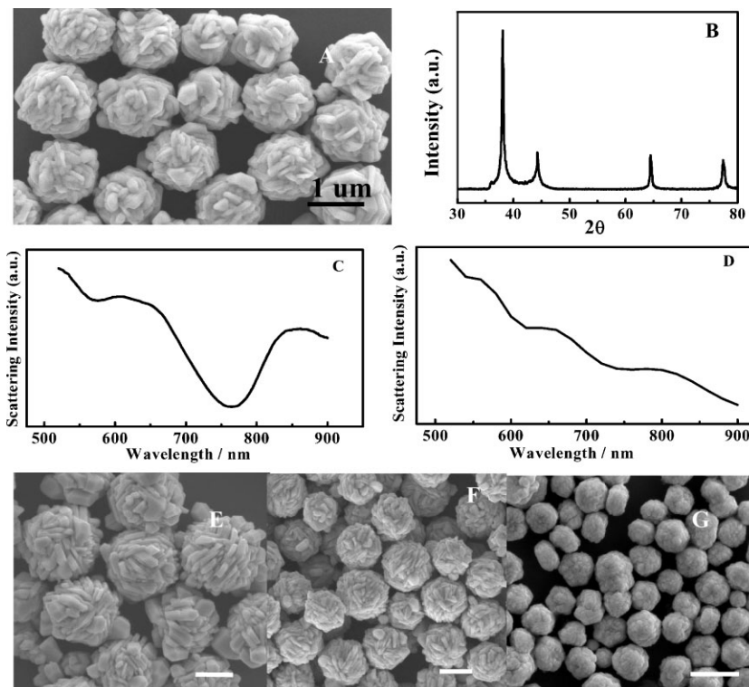
Figure 1. A) SEM image of flower-like silver particles. B) XRD pattern taken from the same batch of sample. C) DF scattering spectrum of a single particle. D) Theoretically calculated scattering spectrum of an Ag sphere with the same size as in the experiment. The multipoles in the simulation is taken up to 40, which is enough for the convergence of the simulation. E–G) SEM images of flower-like Ag particles with different sizes obtained by changing the concentration of silver nitrate in reacting solution. E) 100 \times 10^{-3} M, F) 20 \times 10^{-3} M, and G) 4 \times 10^{-3} M. All scale bars are 1000 nm.
